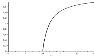
Figure 2. Graph of threshold harvesting function H(N) .
