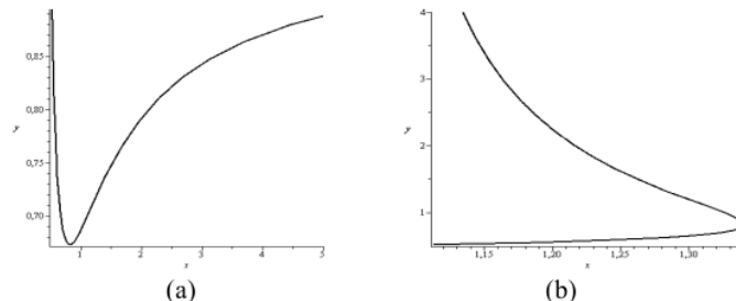
Figure 3. Simple isoclines (a) for dx/dt = 0 and (b) for dy/dt = 0 .
