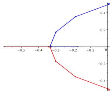
Figure 4. The effect of changing the values of h_1 and h_2 and stability of the equilibrium point.
