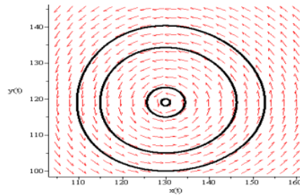
Figure 1. Some trajectories around the equilibrium point E_0 = (130, 119.0476) .
